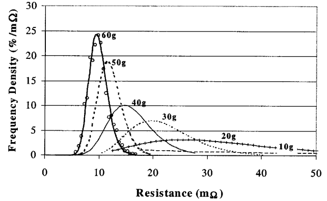
Fig. 7. Inverse Gaussian resistance distributions of electrically conductive elastomer buttons under various contact loads. The experimental data for 60 g contact load (open circle) is compared to the calculated distribution.
