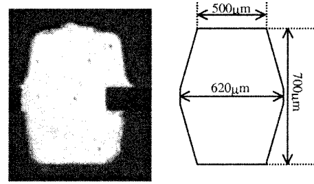
Fig. 1. Cross section of a conductive elastomer button with a schematic displaying the average dimensions.
