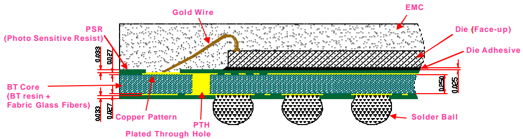
Figure 2. Vertical Structure of a FBGA Package with 2-Layer PCB (courtesy of Samsung)
