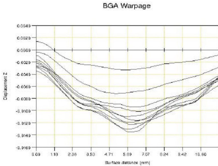
Figure 4: Plots of out-of-plane Displacement along The Diagonal Section Line indicating Warpage.
