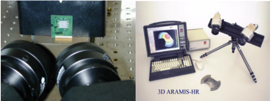
Figure 1. Setup shot showing pair of cameras with 50 mm lenses and built-in macro rings aimed at the prepared ball grid array assembly (left). A 3-D image correlation measurement system (right). (Courtesy of Trilion Quality Systems )
