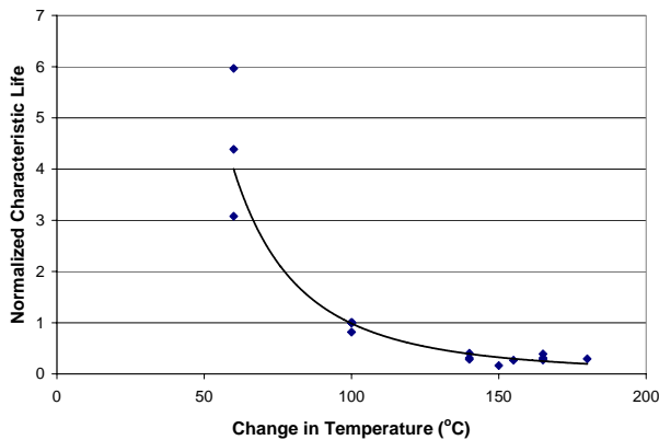
Figure 9: Normalized characteristic lifetime as a function of change in temperature for area array packages (BGA and CSPs)
