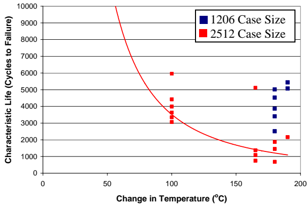
Figure 1: Cycles to failure as a function of change in temperature during thermal cycling for leadless chip resistors attached with SAC solder.
