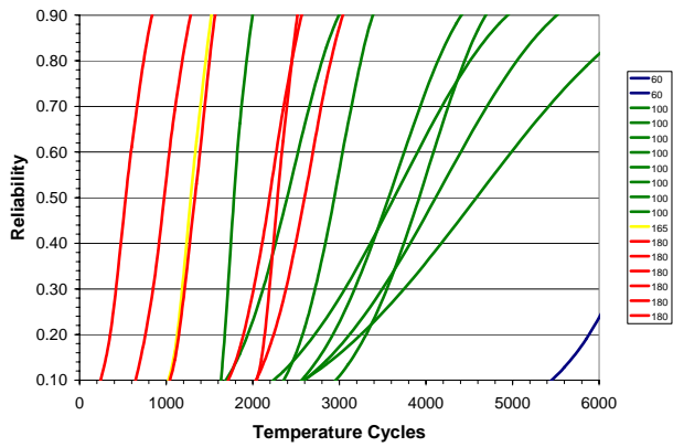
Figure 5: Two parameter Weibull plots of Alloy42 TSOPs attached using SAC solder and subjected to various temperature cycles (40C to 100C: 60; 0C to 100C: 100; -40C to 125C: 165; -55C to 125C: 180).
