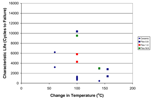
Figure 7: Cycles to failure as a function of change in temperature during thermal cycling for ceramic and flex BGAs attached with SAC solder. Coloration identifies different pitches (0.8 mm, 1.0 mm, unknown).
