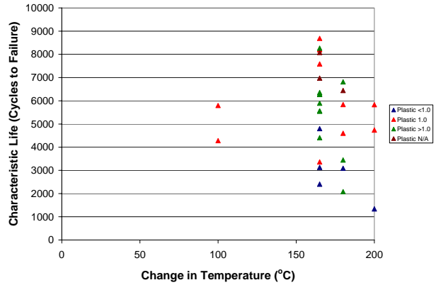
Figure 6: Cycles to failure as a function of change in temperature during thermal cycling for PBGAs attached with SAC solder. Coloration identifies different pitches (less than 1.0 mm, 1.0 mm, greater than 1.0 mm, unknown).
