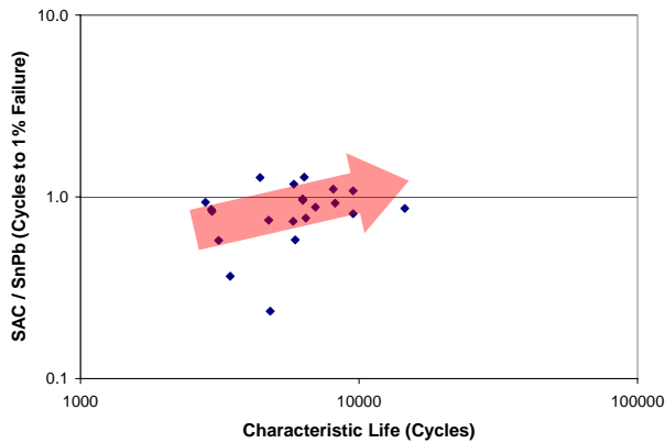
Figure 15: Ratio of SAC/SnPb time to 1% failure for area array devices as a function of characteristic lifetime of the SAC component and taking into account long-term dwell (8 hours).
