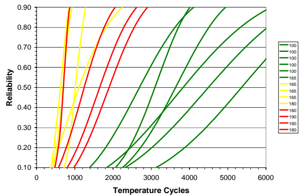
Figure 4: Two parameter Weibull plots of 2512 resistors attached using SAC solder and subjected to various temperature cycles (0C to 100C: 100; -40C to 125C: 165; -55C to 125C: 180).
