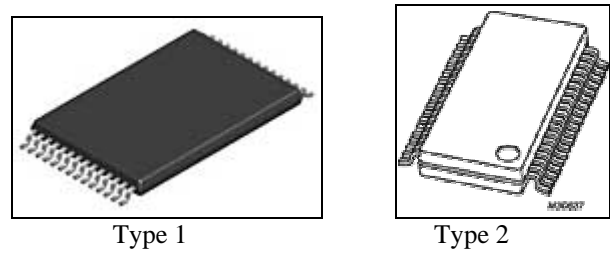
Figure 3: Type 1 and Type 2 TSOP package styles.
