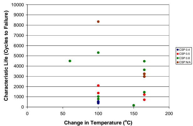
Figure 8: Cycles to failure as a function of change in temperature during thermal cycling for CSPs attached with SAC solder. Coloration identifies different pitches (0.4 mm, 0.5 mm, 0.8 mm, unknown).
