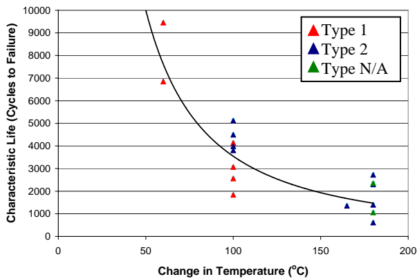
Figure 2: Cycles to failure as a function of change in temperature during thermal cycling for TSOPs with Alloy42 leadframe attached with SAC solder.
