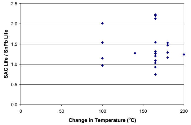
Figure 13: Ratio of SAC/SnPb reliability for area array devices as a function of change in temperature.
