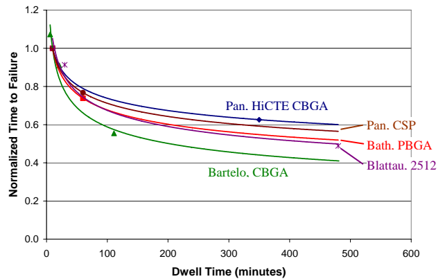
Figure 10: Normalized time to failure as a function of dwell time at maximum temperature for SAC solder.
