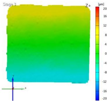
Figure 14: Bottom Y deformation at 70°C
