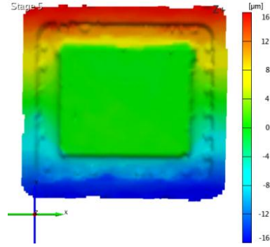
Figure 11: Top Y deformation at 110°C
