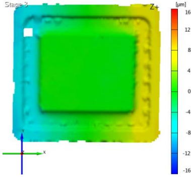
Figure 8: Top X deformation at 70°C
