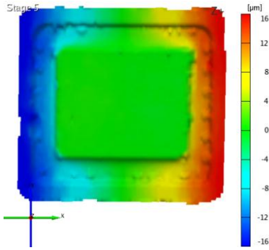
Figure 9: Top X deformation at 110°C
