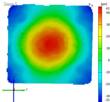
Figure 17: Warpage at 110°C
