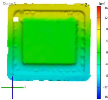
Figure 10: Top Y deformation at 70°C
