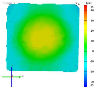
Figure 16: Warpage at 70°C
