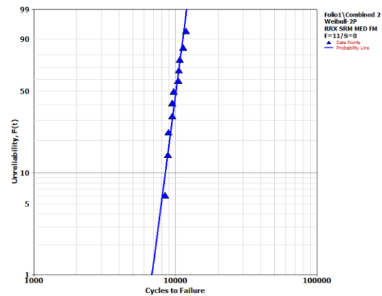
Figure 7: Cycles to failure for both samples combined into one Weibull
