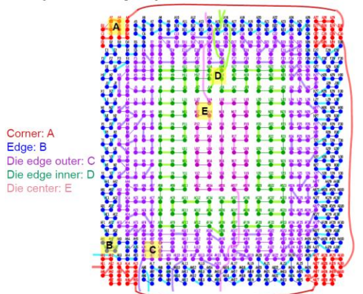
Figure 3: Daisy chain locations
