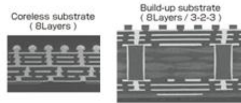
Figure 1: Coreless substrate (left) and standard substrate 1
