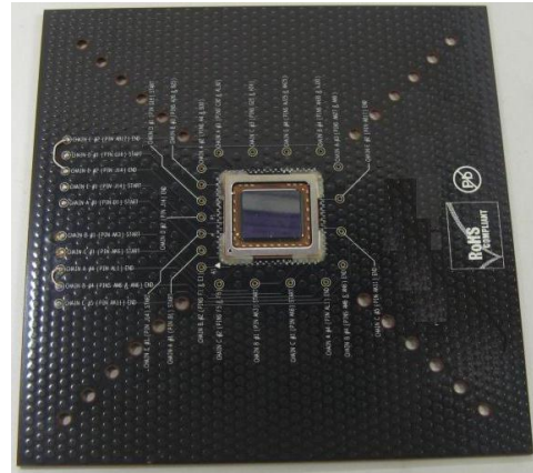
Figure 4: Test PCBA
