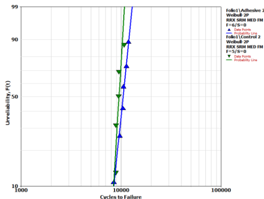
Figure 6: Cycles to failure for samples with (green) and without (blue) edge bonding
