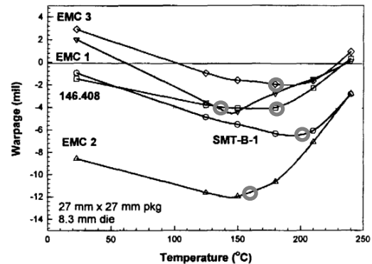
Figure 18: Warpage of molding compounds; grey circles indicate approximate T_g [1]
