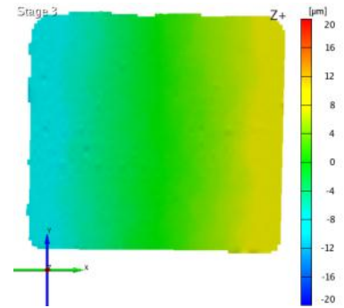
Figure 12: Bottom X deformation at 70°C
