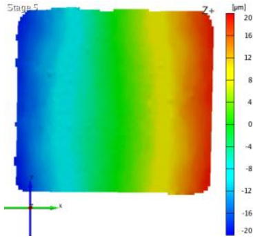
Figure 13: Bottom X deformation at 110°C
