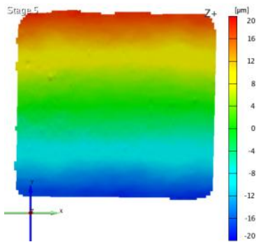
Figure 15: Bottom Y deformation at 110°C
