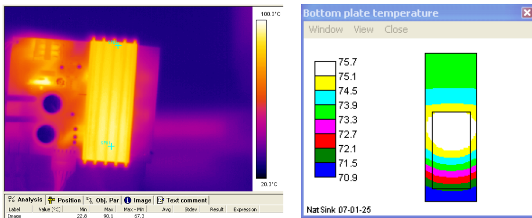
Figure 3: Heatsink temperatures at 20°C ambient
