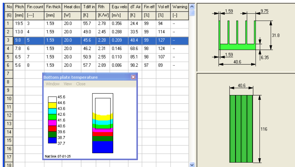
Figure 6: Heat source located near top
