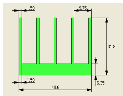
Figure 2: Dimensions of heatsink
