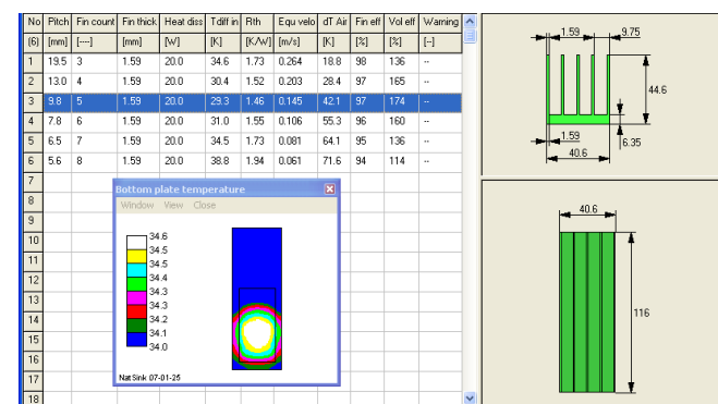
Figure 10: Emissivity increase with +0.5" fins, 13.8°C drop
