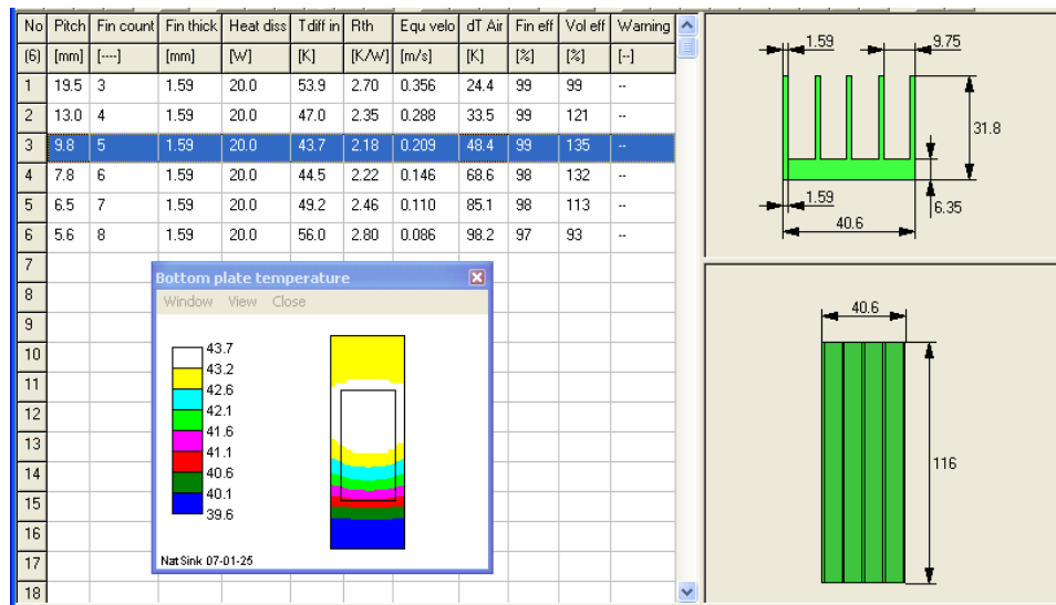
Figure 5: Heat source located at center
