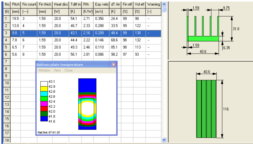
Figure 4: Baseline heatsink analysis at 20 watts, 60°C ambient, five fins optimal, 103°C
