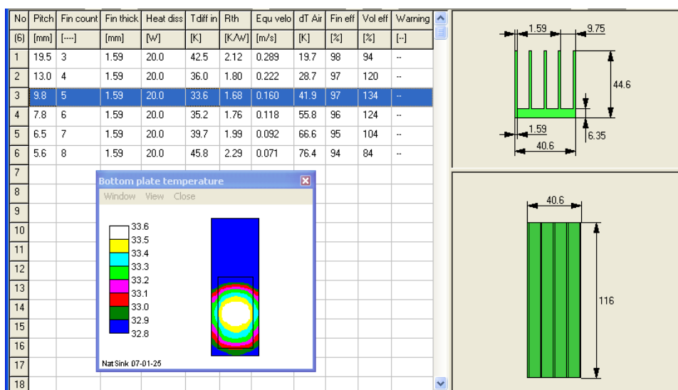
Figure 8: Heatsink fin height +0.50"
