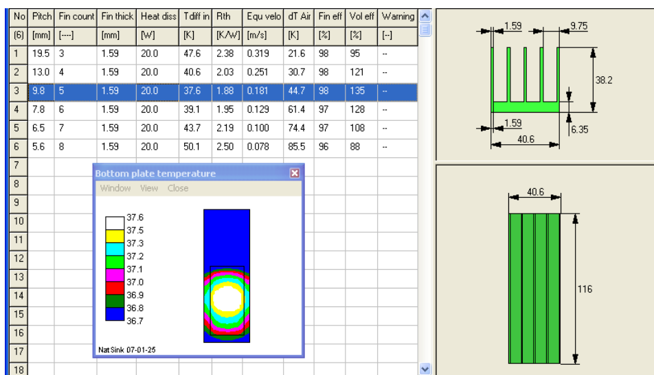
Figure 7: Heatsink fin height +0.25"
