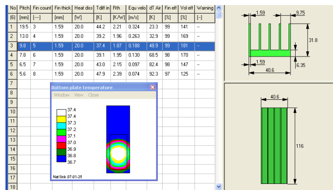
Figure 9: Emissivity increase, 5.7°C drop
