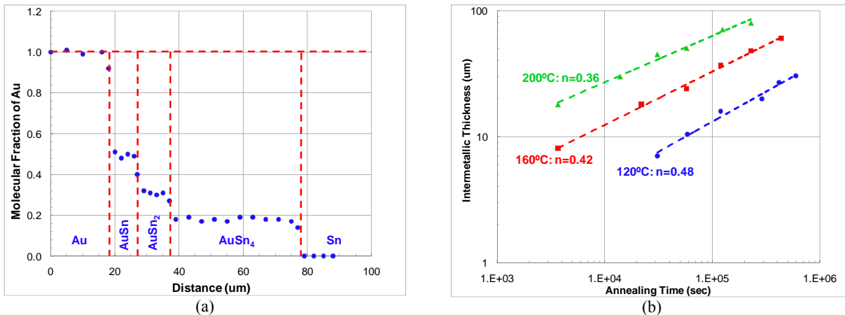
Figure 4: (a) Intermetallic formation in Au-Sn diffusion couple after 127 hrs at 160°C [39]; (b) total intermetallic thickness ( \text{AuSn}_4 + \text{AuSn}_2 + \text{AuSn} ) as a function of annealing time at different temperatures, with the associated time exponent in Equation 1 [31,39].
