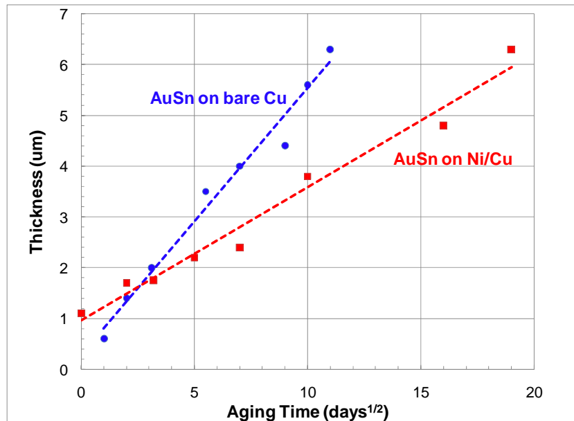
Figure 2: Consumption of barrier metallization by intermetallic versus time at 200°C for eutectic AuSn solder on Ni UBM and bare Cu [19,40].
