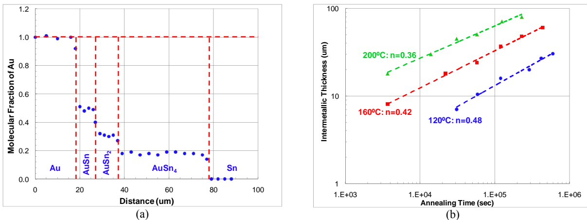
Figure 4: (a) Intermetallic formation in Au-Sn diffusion couple after 127 hrs at 160°C [39]; (b) total intermetallic thickness ( AuSn_4 + AuSn_2 + AuSn ) as a function of annealing time at different temperatures, with the associated time exponent in Equation 1 [31,39].
