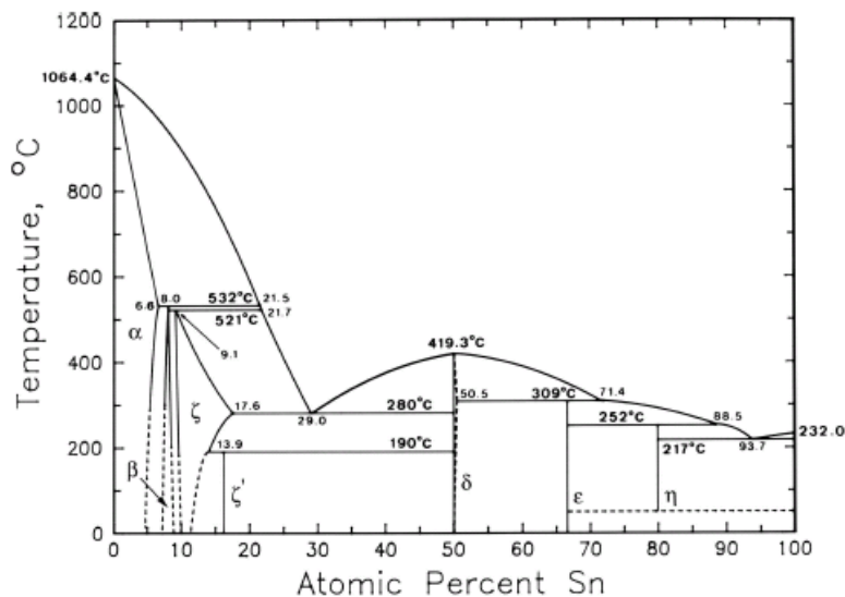
Figure 1: Au-Sn binary phase diagram (adapted from [1]).
