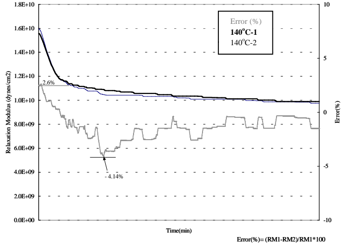
Figure 12. 0.5% Strain Application in Repeatability Test (RM: Relaxation Modulus)
