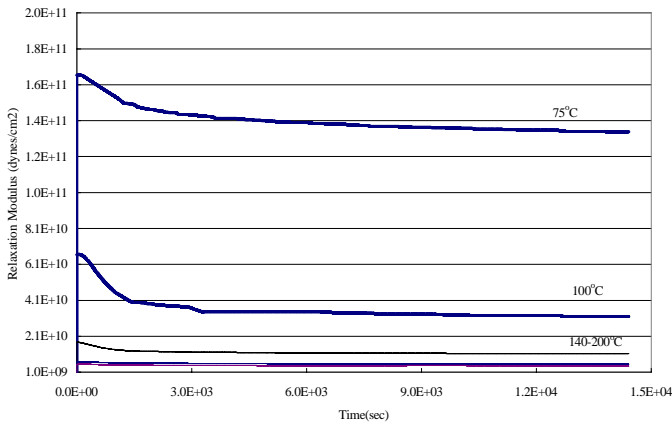
Figure 11. Relaxation Modulus of 0.25% Strain Application at 75-200°C
