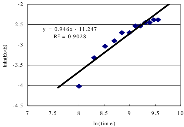
Figure 6. \ln\ln(E_0/E) versus \ln(\text{time}) under 0.1% Strain Application at 75°C
