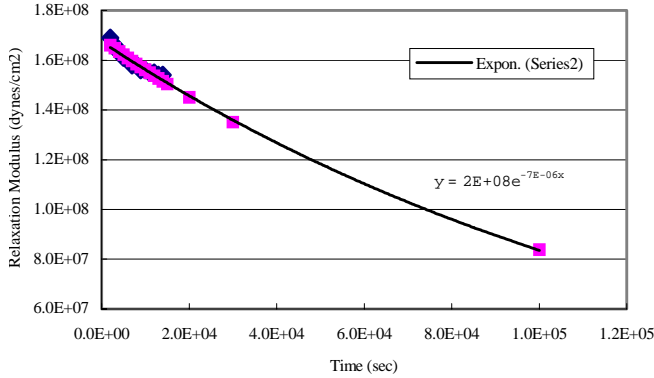
Figure 5. Curve Fitting of Relaxation Modulus under 0.1% Strain Application at 75°C
