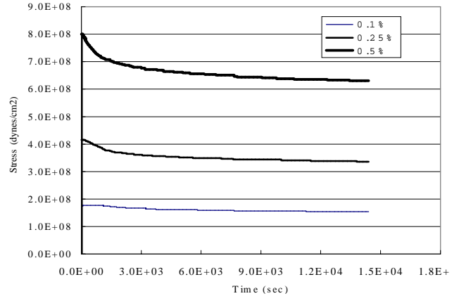
Figure 3. Stress Relaxation Curves at 0.1-0.5% Strains at Reference Temperature of 75°C
