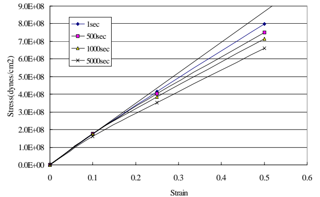
Figure 4. Non-linear Relation of Stress vs. Strain at 75°C
