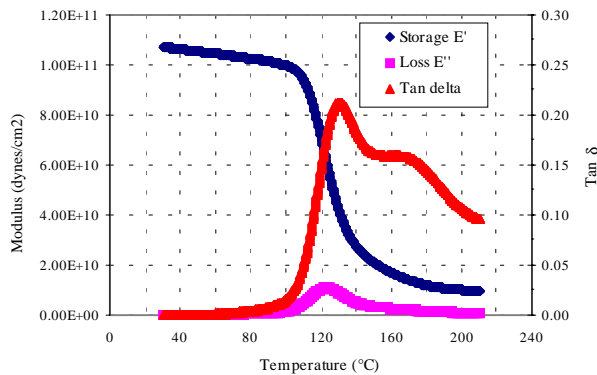
Figure 1. Viscoelastic Modulus of Plastic Molding Compound
