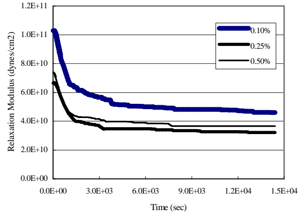
Figure 7. Relaxation Modulus vs Time of 0.1, 0.25, and 0.5% Strains at 100°C
