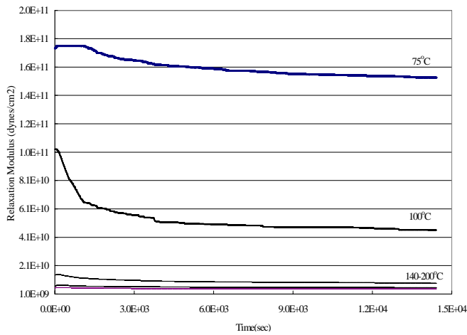
Figure 10. Relaxation Modulus of 0.1% Strain Application at 75-200°C
