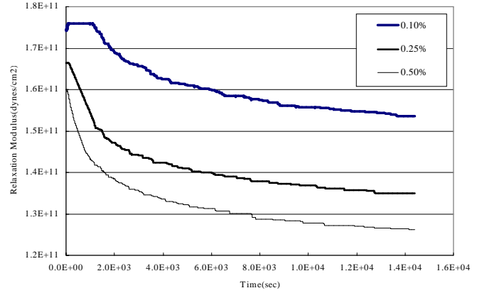
Figure 2. Relaxation Modulus Curves at 0.1-0.5% Strains at Reference Temperature of 75°C
