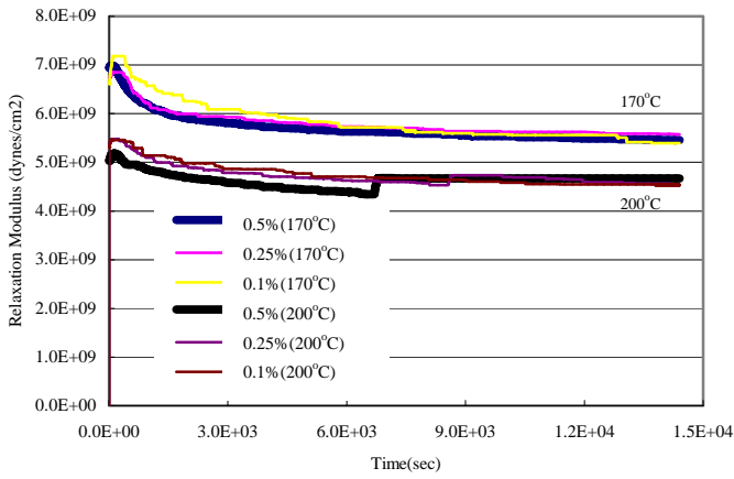
Figure 9. Relaxation Modulus at 170°C and 200°C in 0.1, 0.25, and 0.5% Strain Application
