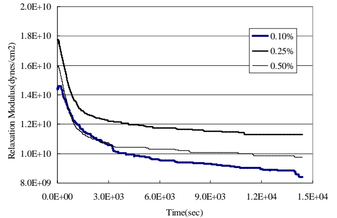
Figure 8. Relaxation Modulus vs Time of 0.1, 0.25, and 0.5% Strains at 140°C
